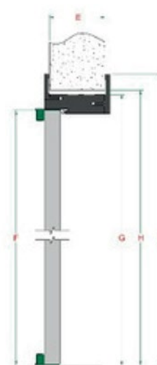
Section verticale
